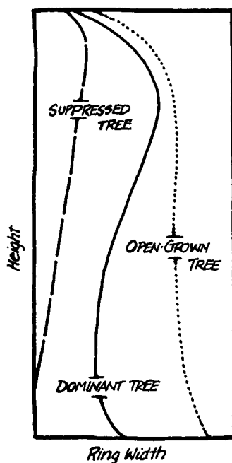
Variations in thickness of the annual ring at various stem heights.
